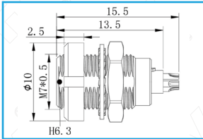
ECG(双螺母安装)
